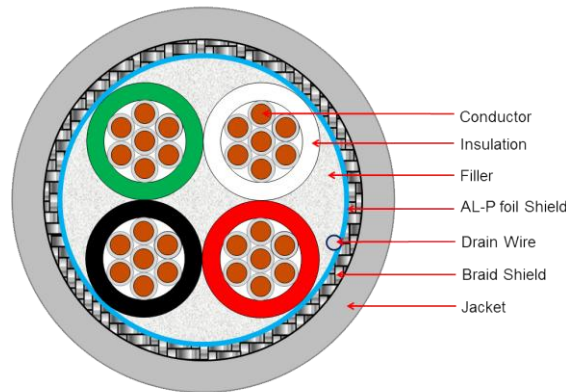
LINK Multi-Core cable, 4 cores Double Shield
