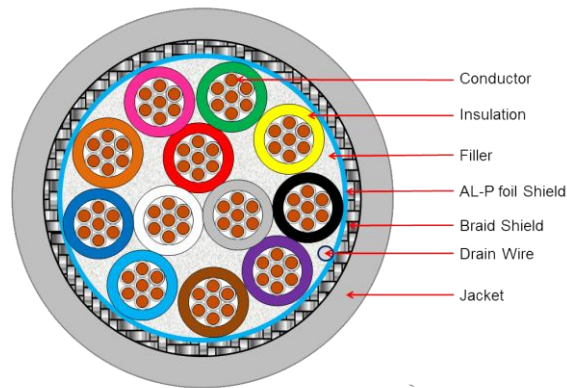
LINK Multi-Core cable, 12 cores Double Shield
