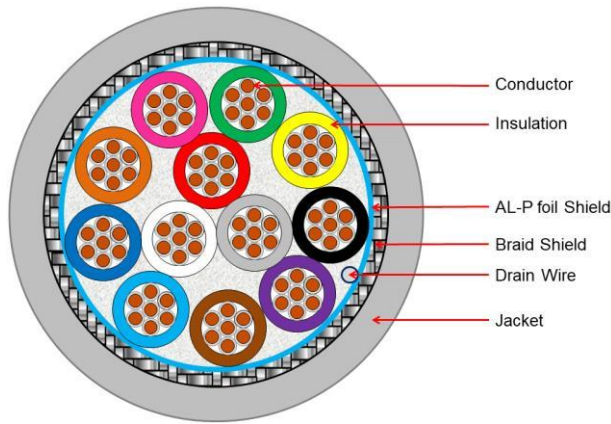
LINK Multi-Core cable, 12 cores Double Shield
