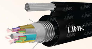
Fig.8, Multi-Tube, Armored UFCX8XXMA
