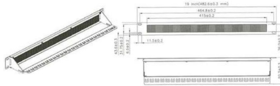
US-3055 Brush Cable Management with Management bar
